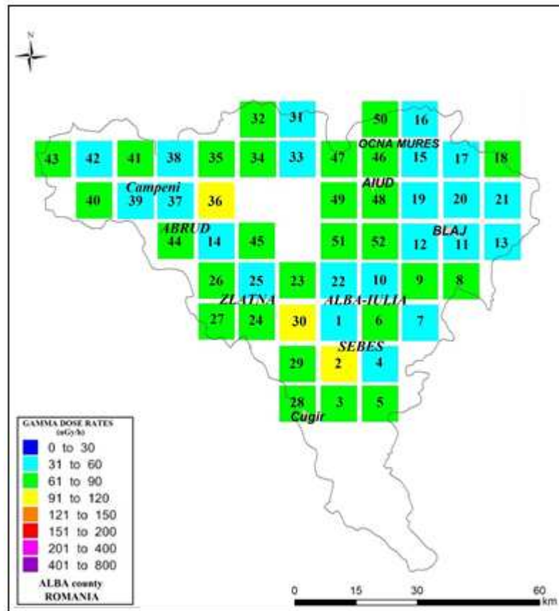
Figure [1]. The high resolution map of gamma dose rates [nGy/h] for Alba County, Romania (the codes within every cell are given in Table 1).
